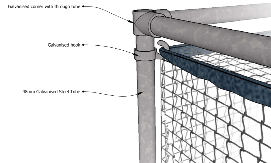
TOP CORNER DETAIL scale: NTS
