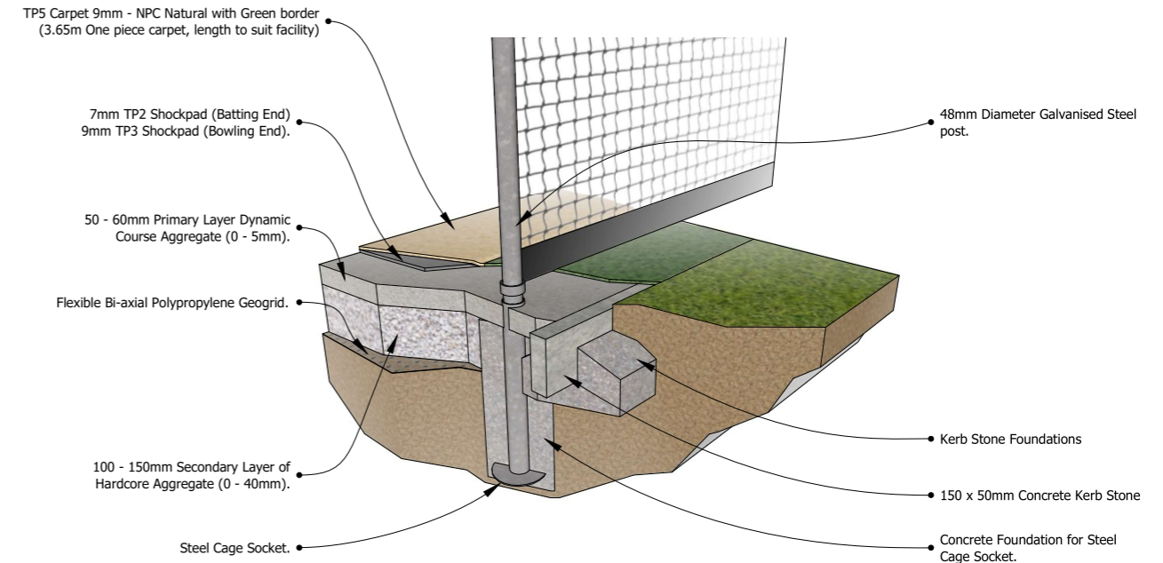
CAGE POST INSTALLATION scale: NTS
